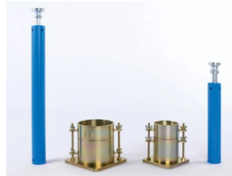
Standard Soil Proctor With Mould
