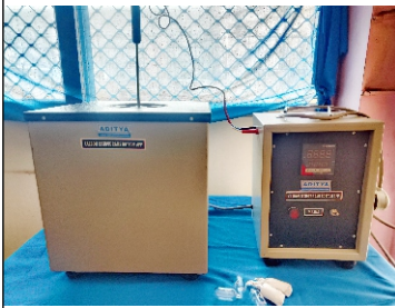
Carbon Residue Ramsbottom App
