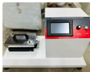
Constant Head Geotextile Permeability Test Apparatus
