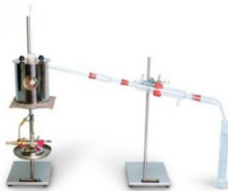
Distillation For Cut Back Bitumen
